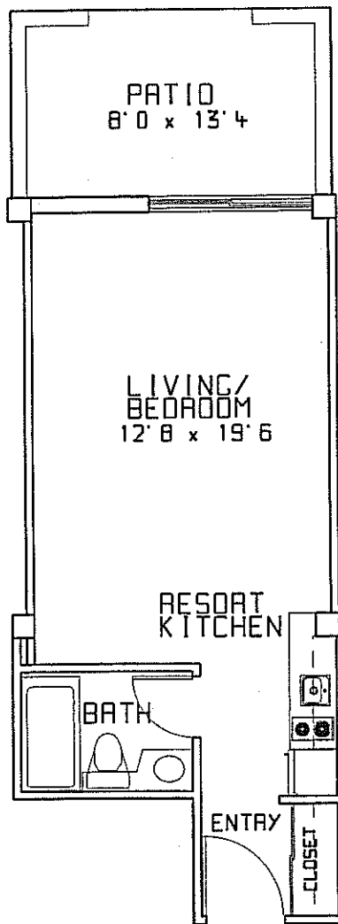
UNIT TYPE F 445 SF. TYPICAL OF UNITS 104-106
