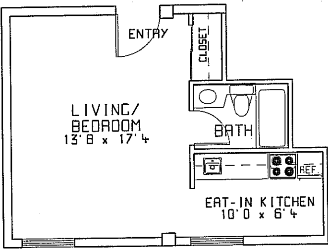
UNIT TYPE Q 356 SF. TYPICAL OF UNITS 220-320-420-520 620-720-820
