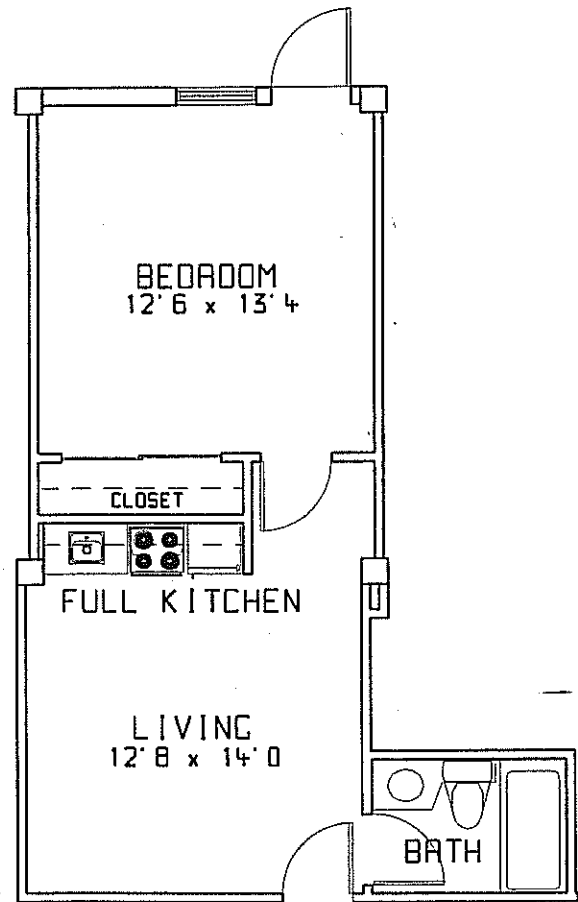
UNIT TYPE B 412 SF. TYPICAL OF UNITS 105-107-113
