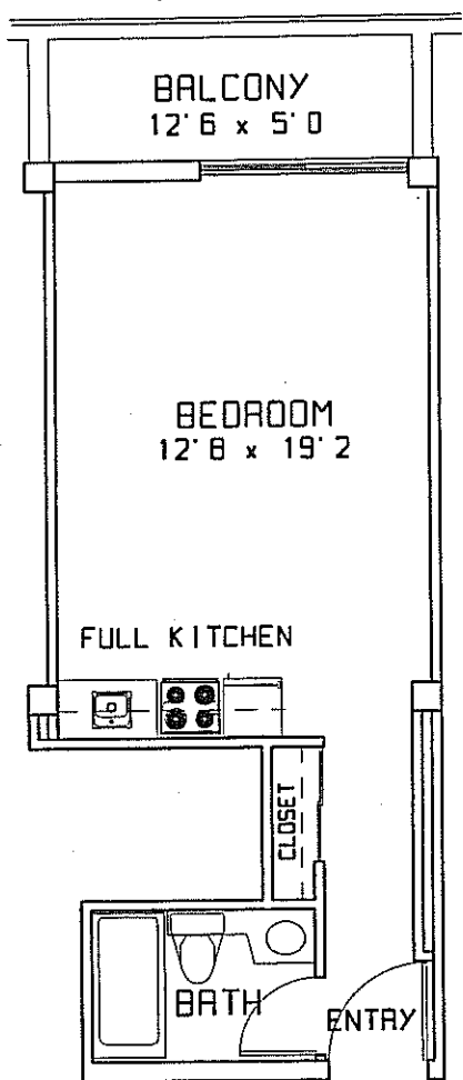
UNIT TYPE H1 377 SF. TYPICAL OF UNITS 502-602-702-802
