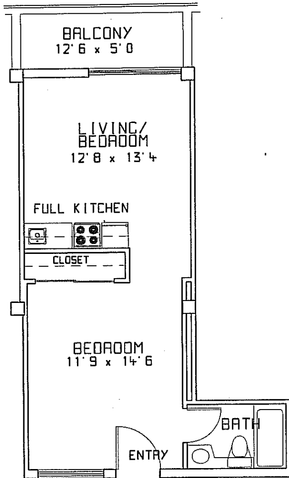
UNIT TYPE M 402 SF.
