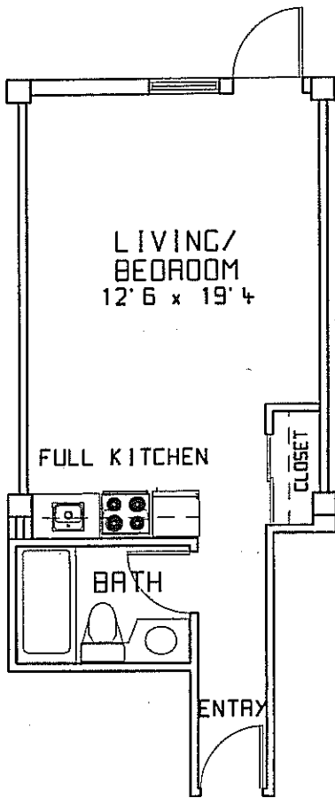
UNIT TYPE C 309 SF. TYPICAL OF UNIT 112
