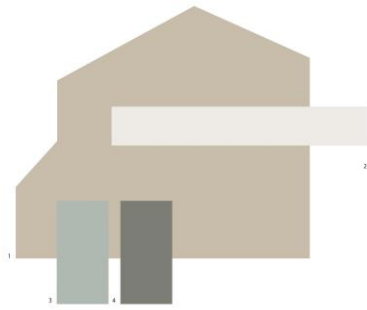
Scheme 10
