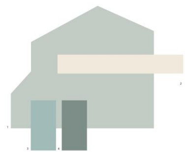
Scheme 12
