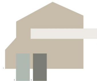
Scheme 10
